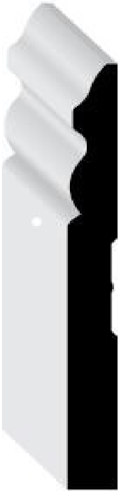
5180 BASE 9/16 X 5-1/4 Primed FJ or LDF
